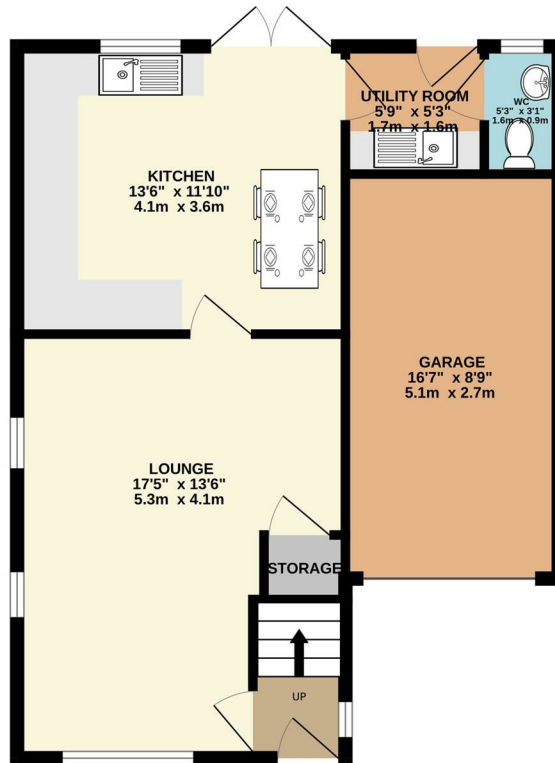
GROUND FLOOR 586 sq.ft. (54.4 sq.m.) approx.
